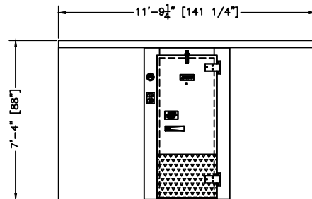
ELEVATION SHOWN W/ RIGHT HINGE (LEFT HINGE AVAILABLE)
