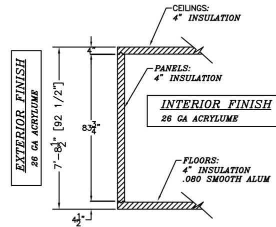
SECTION WALL WITH FLOOR
